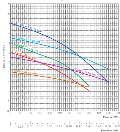
Performance for Pump in DN-80mm
